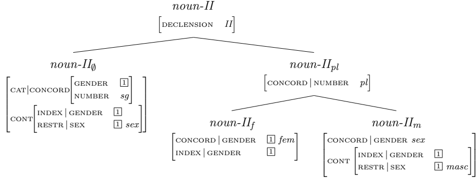
Figure 2: Revised version of the class II type hierarchy
